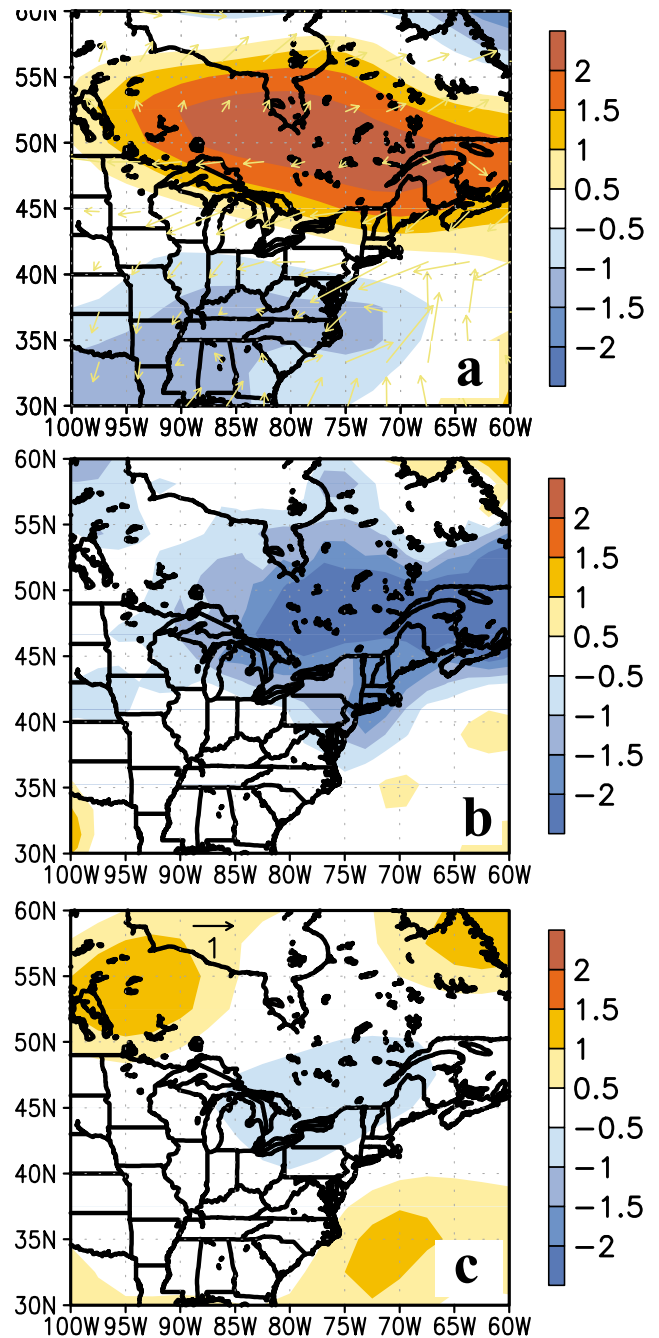
Fig. 14. April-June 2003 anomalous (a) sea-level pressure (hPa) and vector wind, (b) 1000-hPa temperature ( ^\circ\text{C} ), and (c) 925 hPa temperature ( ^\circ\text{C} ). Anomalies are departures from the 1971-2000 base period means.
